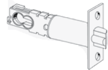
16-126 Dead Latch Square Corner 5" BS
