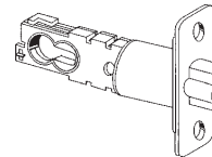
16-207 Dead latch Square corner 2-3/8" or 2-3/4" BS with A501-878 Front Adapter
