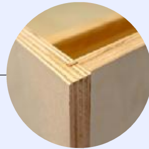
Full 3/4" Thick Plywood Back Panel
